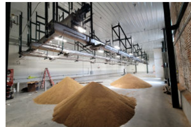
Food Products Such as Spent Grains are Easily Handled with Screw Conveyors
