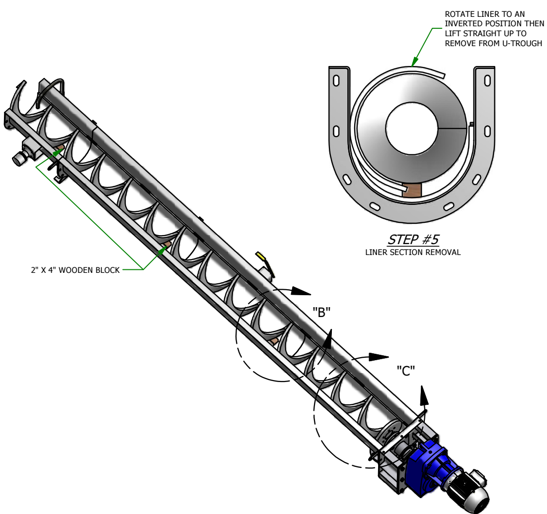
STEP #4 LIFT AND SUPPORT SPIRAL
