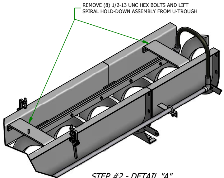
STEP #2 - DETAIL "A" HOLD-DOWN REMOVAL
