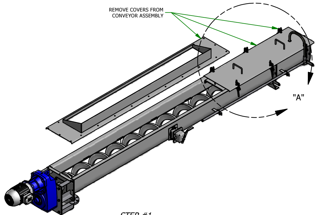
STEP #1 COVER REMOVAL
