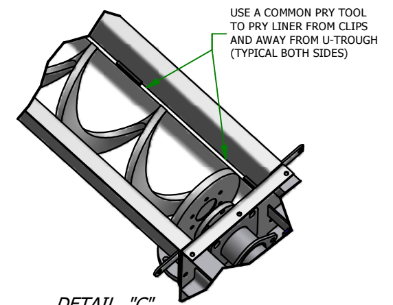
DETAIL "C" LINER REMOVAL
