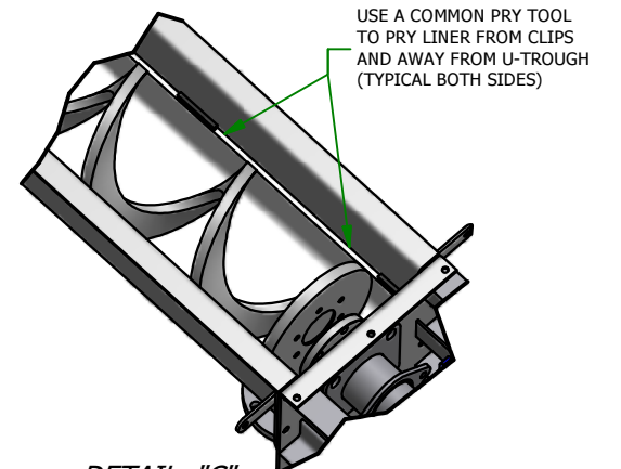
DETAIL "C" LINER REMOVAL
