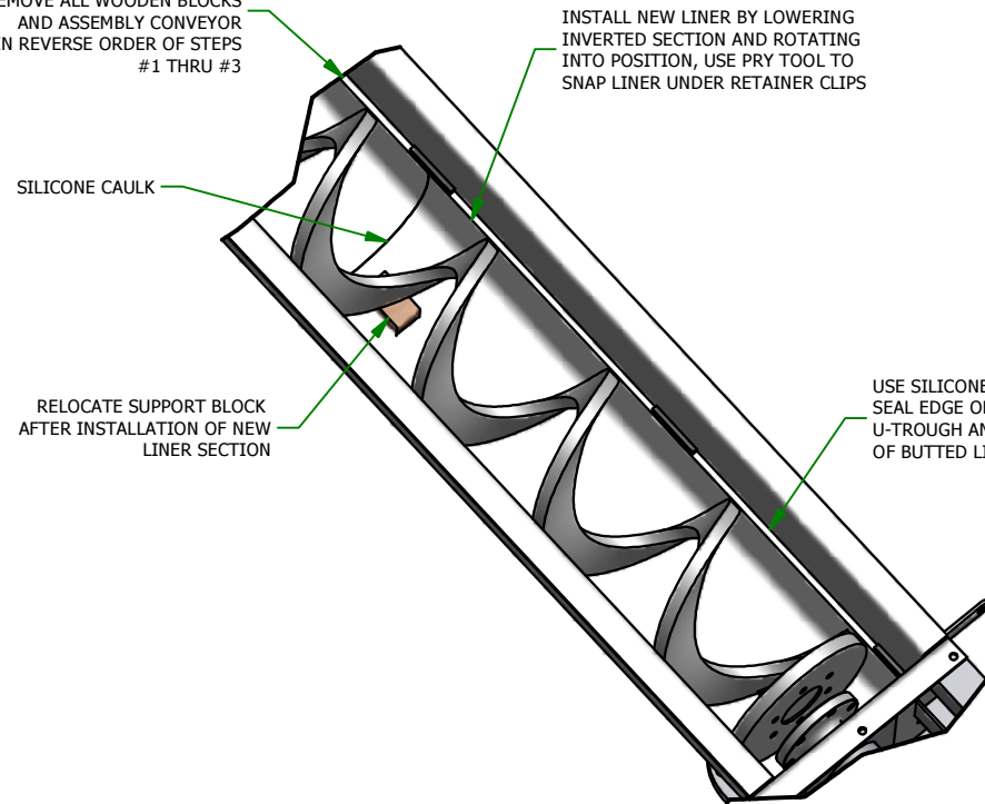
STEP #6 NEW LINER INSTALLATION
