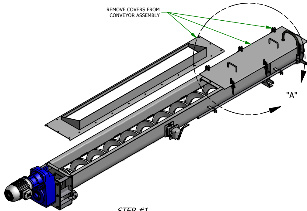
STEP #1 COVER REMOVAL
