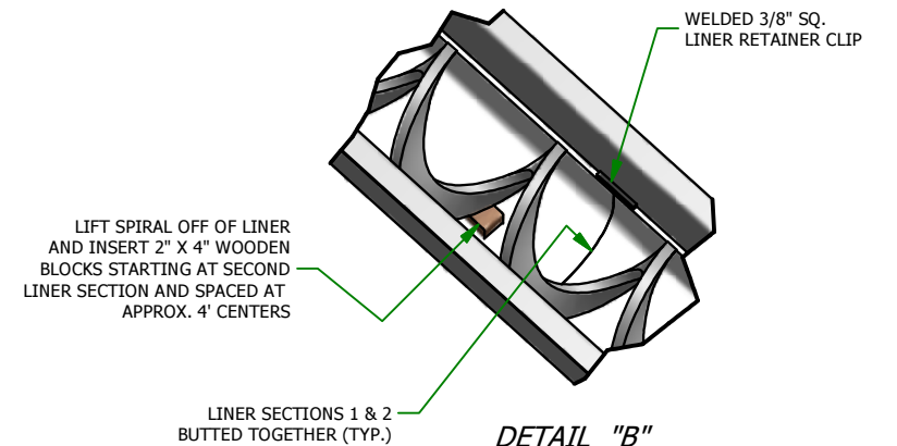
DETAIL "B"
