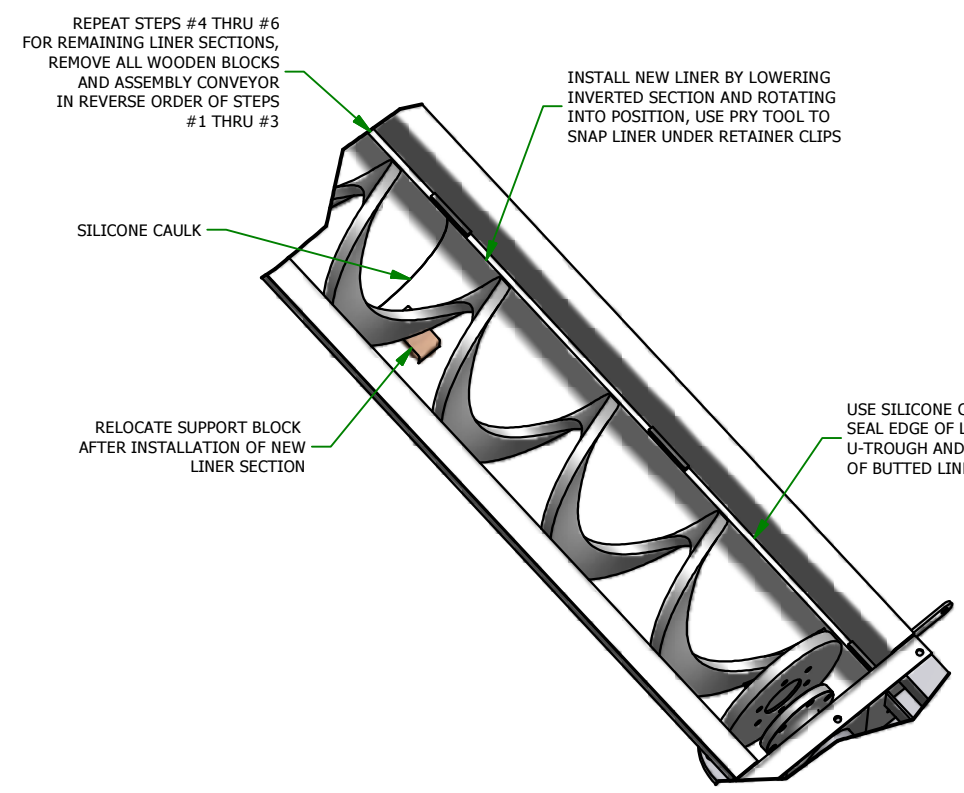
STEP #6 NEW LINER INSTALLATION
