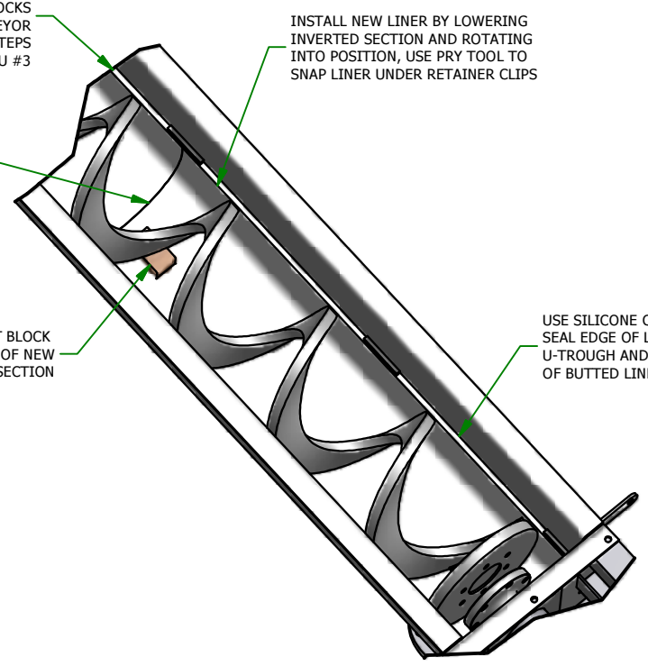
STEP #6 NEW LINER INSTALLATION
