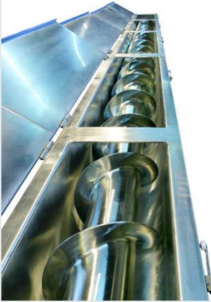
Hinged Covers with Quick-Release Clamps Allow for Easy Cleaning of Internal Surfaces
